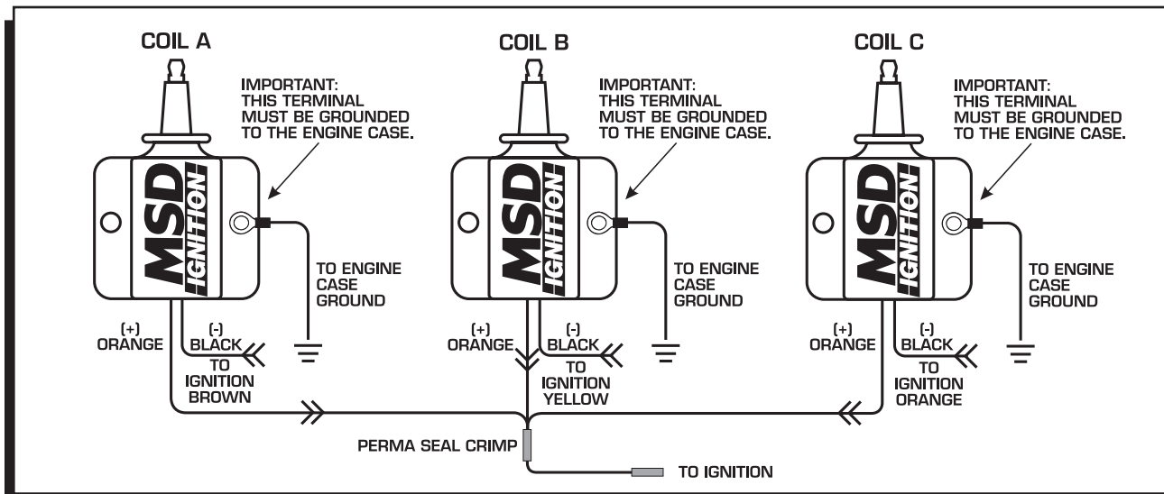
Figure 3 Triple Coil System Used with PN 42351 Ignition.
